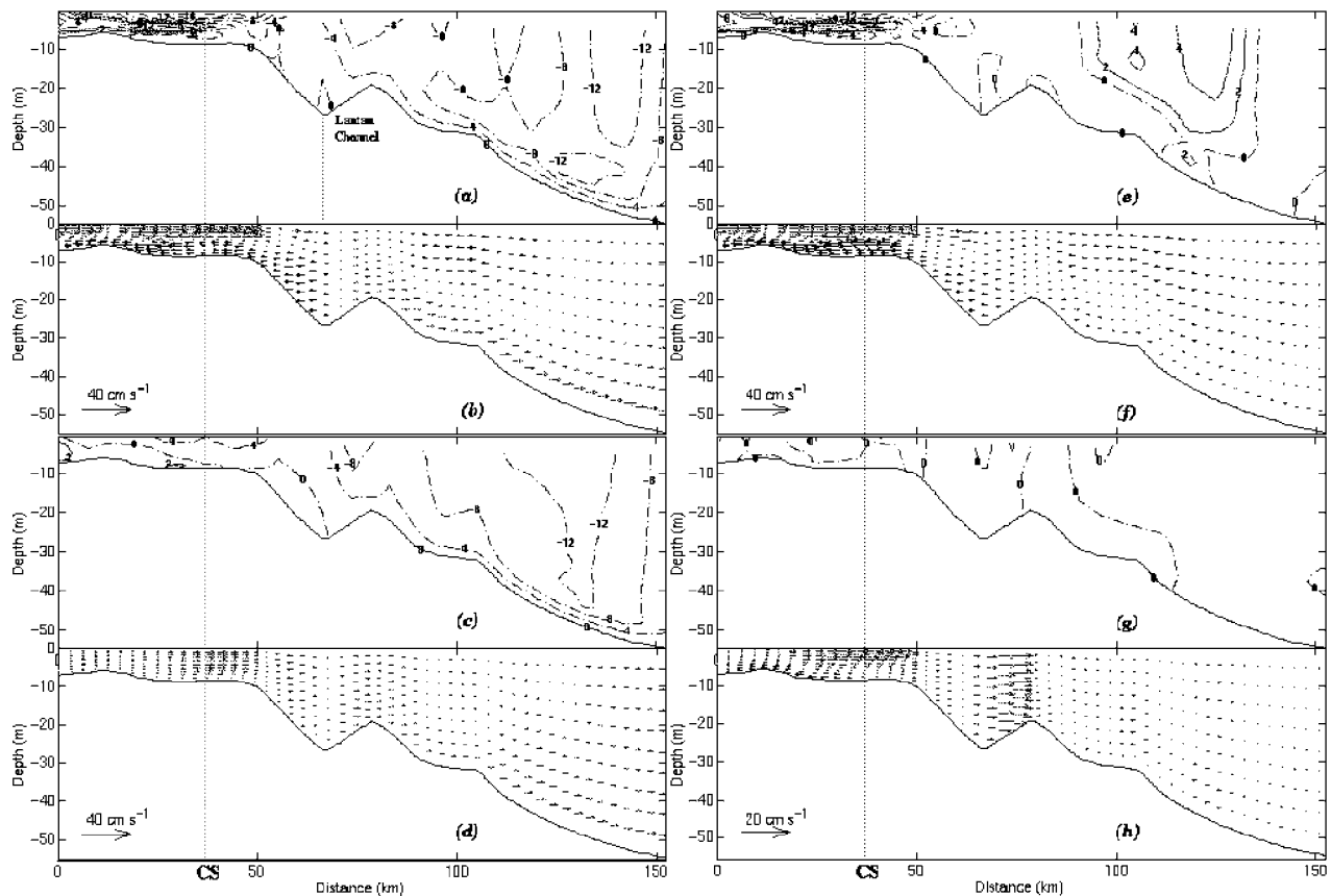
Figure 4. The comparison of the vertical distribution of the winter horizontal circulations along the cross section AL. (a) and (b) The total subtidal circulation, (c) and (d) the “barotropic” component of the subtidal circulation, (e) and (f) the “baroclinic” component of the subtidal circulation, and (g) and (h) for the subtidal circulation during the spring tide due to nonlinear tidal effects. Figures 4a–4f correspond to the neap tide.
