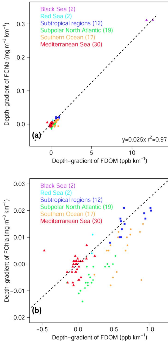
Fig. 6. Scatter plots of the depth-gradients of FChla and depth-gradients of FDOM of all 82 Bio-Argo floats with the black dashed line representing the linearly regressed line ( y=0.025x , r^2=0.97 ). Each point represents the averaged value of all profiles observed by each float.
