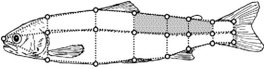
FIGURE 1.—Schematic of an Atlantic salmon smolt and the landmarks used to estimate surface area. Shaded area represents the area descaled as a standardized injury in this study.
