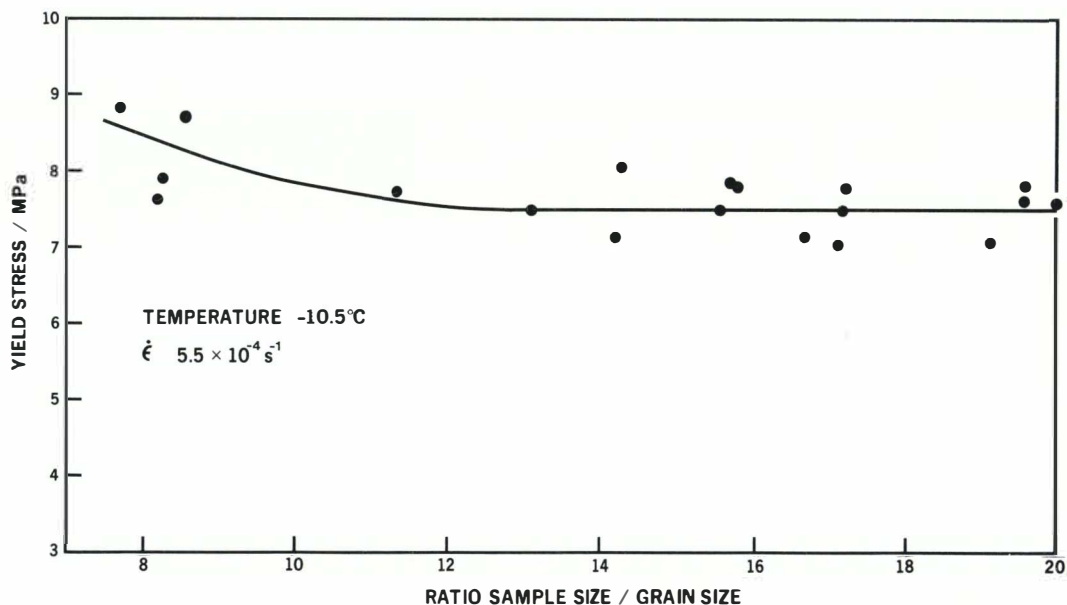
Fig. 2. The maximum yield stress plotted against the ratio of sample size to grain-size. The grain-size was kept constant at 1.0 mm and the sample diameter was varied. Below a ratio of 12 the yield stress depends on this ratio.
