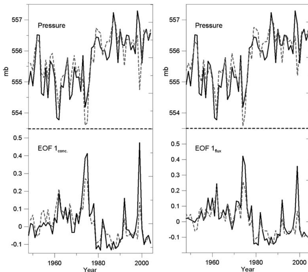
Figure 5. Plots of annual pressure and EOF I_{\text{conc. and flux}} (solid line) and their common EOF 1 (dashed shaded line). For positive correlations (e.g., EOF I_{\text{conc.}} and EOF I_{\text{flux}} ), the EOF is oriented inversely.
